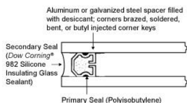
Figure 1: Dual-Seal Type
